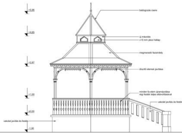
WEST VIEW
