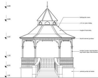
SOUTH VIEW
