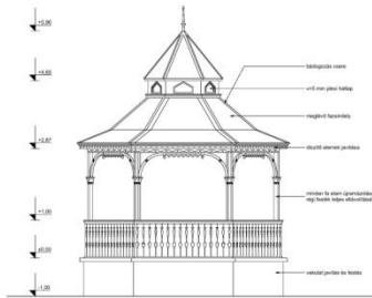
NORTH VIEW
